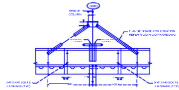
THE GIP SHORT LAP DETAILS
