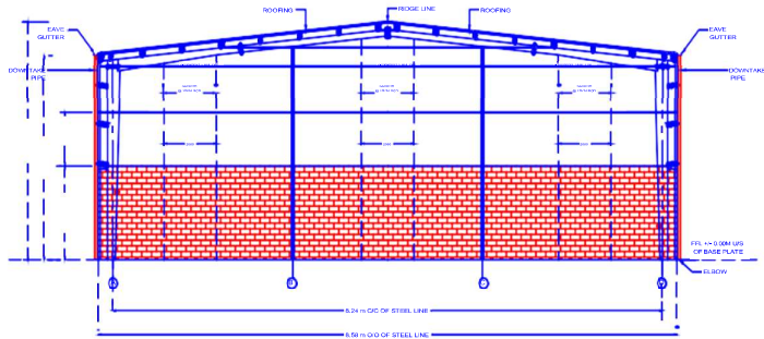
END WALL FRAMING ELEVATION FOR FRAME LINE 1
