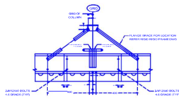
THE GRIP SHORT LAP DETAILS
