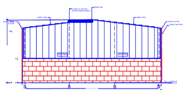
ENDWALL SHEETING ELEVATION FOR FRAME LINE 1
