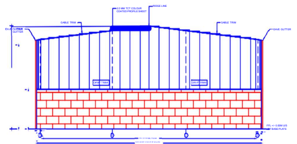
ENDWALL SHEETING ELEVATION FOR FRAME LINE 2
