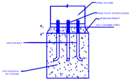
SAMPLE DETAILS OF MINIMUM PEDESTAL REQ FOR PINNED BASE FOR ALL LEAN TO COLUMN
