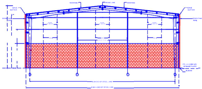
END WALL FRAMING ELEVATION FOR FRAME LINE 2
